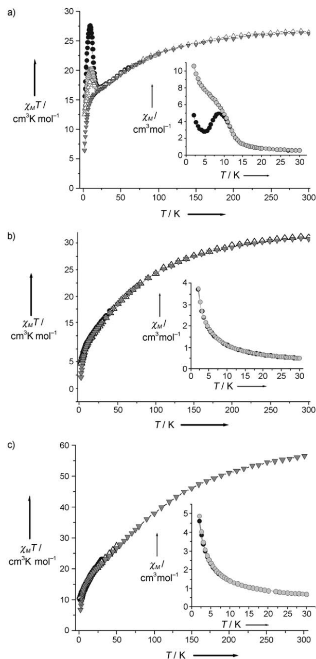
Figure 4. \chi_M T versus T measured in 1 T (▼), 0.1 T (△), 0.05 T (●), or 0.01 T (●) applied fields for a) 1 , b) 2 , and c) 3 . Insets: field-cooled (●) and zero-field-cooled (○) curves measured in 0.01 T applied fields.
